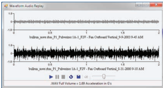
Compare the audio from two different waveforms with the Waveform Audio Replay option.
