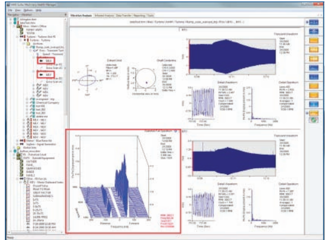
With Cascade Full Spectrum, the user can quickly differentiate between a rub and an oil swirl anomaly.
