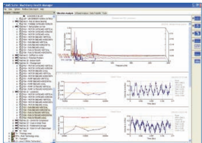
View a complete machine at one time and customize your plot view by selecting what you want to see on the screen. This view shows spectrum, waveform, and trend plots.
