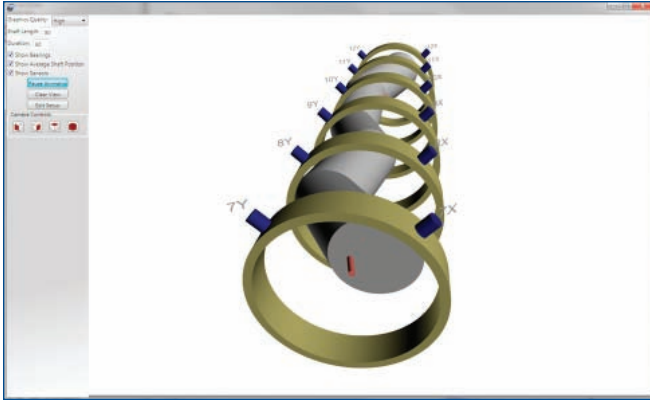
Live 3D shaft animation plots show the actual motion of the shaft around the average shaft position.
